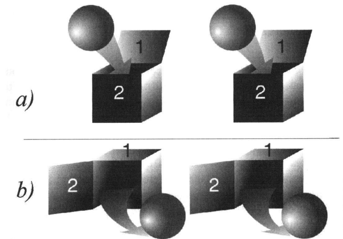
Fig. 1. If you put a ball in a quantum box (A), and then open the wrong door of the box (B), the color of the ball that comes out is random
