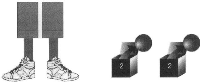
Fig. 2. Classical and quantum correlations
