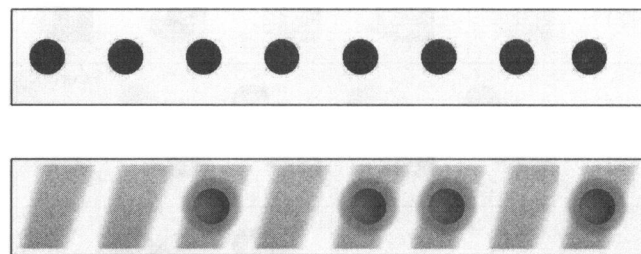
Fig. 7. Reading out quantum information in an ion trap. When the laser is turned on, the red balls glow, and the green balls remain dark.
