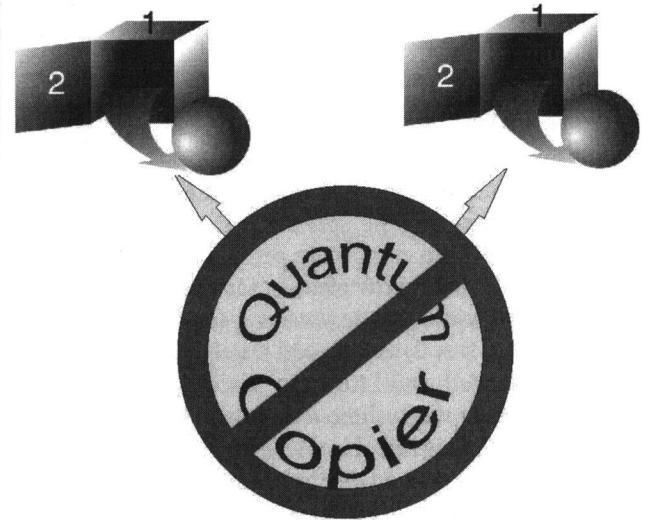
Fig. 5. Quantum information cannot be copied perfectly
