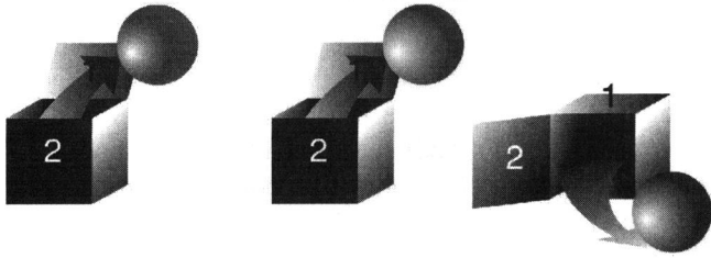
Fig. 3. A quantum correlation among three boxes
